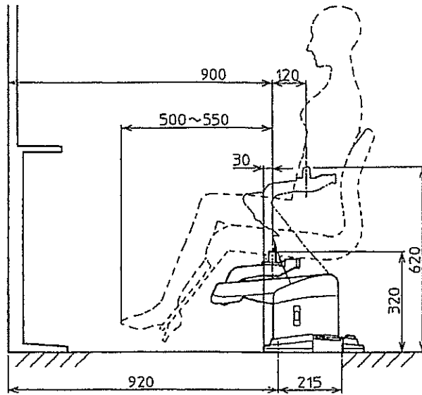
Fig.3-1 Chair Setting Position
