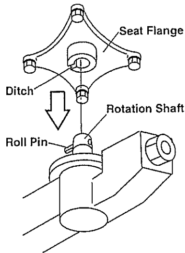
Fig.3-4 Setting Upper Section
